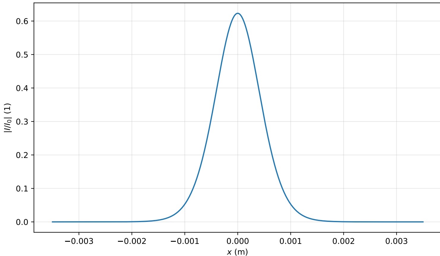
Intensity profile I(x, y = 0, z = 2.388m)/I_0 , P_{in}=0.4P_{cr} , artificial time
